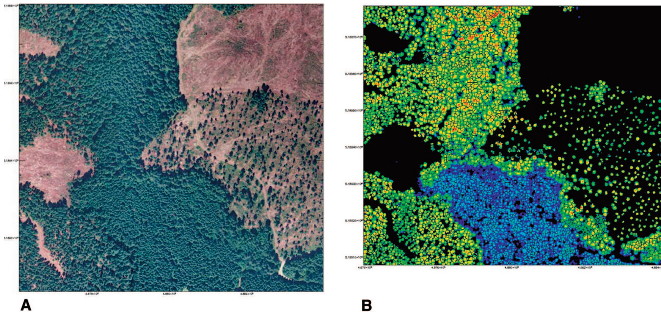
Figure 2. (A) Orthophotograph of selected area (courtesy of Washington Department of Natural Resources), and (B) individual tree-level segmentation of the LIDAR canopy height model via morphological watershed algorithm (color-coded by height; black lines indicate boundaries around crowns).
