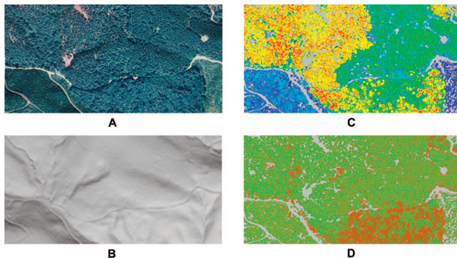
Figure 6. Comparison of a traditional color orthophotograph to LIDAR-derived images for the same area: (A) orthophotograph; (B) bare-ground DEM; (C) CHM (canopy height is less than 2 m in gray areas); and (D) canopy cover image colored by leaf-off LIDAR intensity, where brown low-intensity areas indicate hardwood cover and green high-intensity areas indicate conifer cover.
