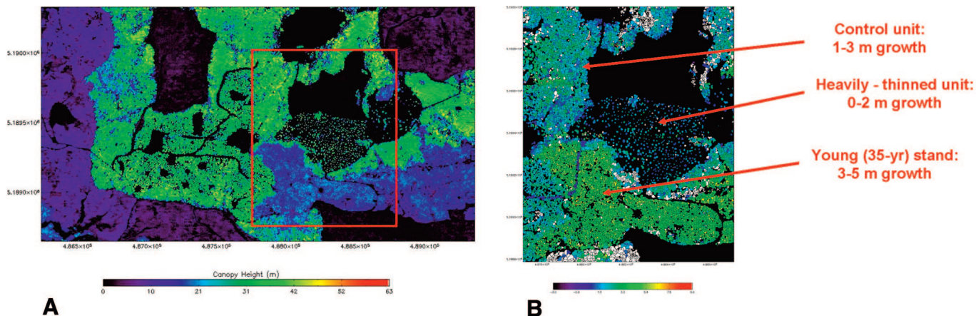
Figure 4. LIDAR-based measurement of individual conifer tree growth (1999–2003). (A) Selected area within Capitol State Forest study area shown in LIDAR canopy height model color-coded by canopy height, and (B) LIDAR-derived individual tree height growth measurement color-coded by height growth. A significant difference in height growth between stands is evident [control (75-year-old, unthinned stand) approximately 1–3 m in growth; young (35-year-old stand) approximately 3–5 m; heavily thinned (75-year-old stand) approximately 0–2 m]. Segments colored white indicate hardwoods that were excluded from this conifer growth analysis.
