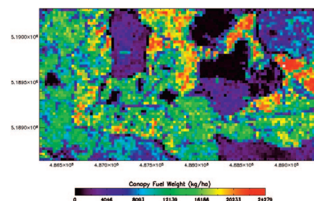
Figure 5. LIDAR-derived canopy fuel weight map (30-m resolution), Capitol State Forest study area (Andersen et al. 2005b).
